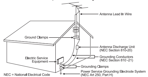
Example Of Antenna Grounding
